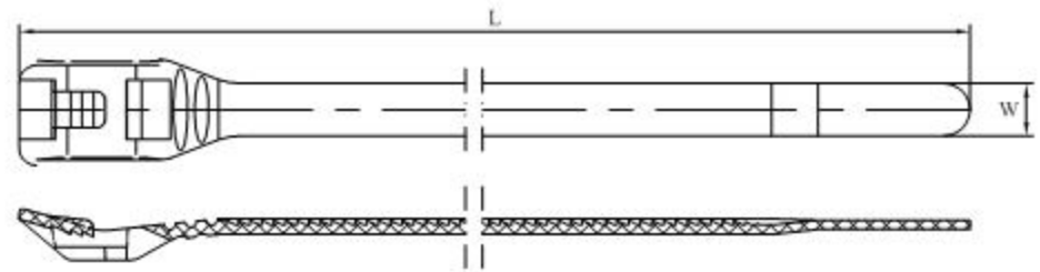
不锈钢嵌片扎带 Stainless Steel Plate Lock Cable Tie
